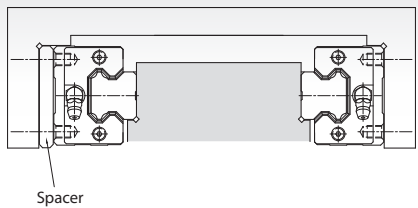
Opposed (Code : F)
