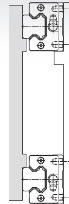
Wall mounting (Code : K)
